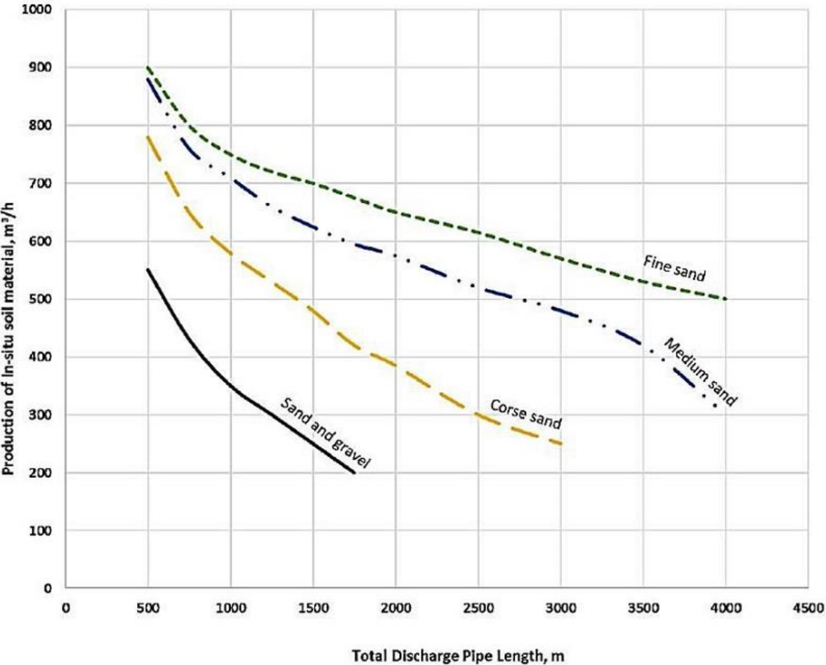
CSD450 - G2 Production Curve
